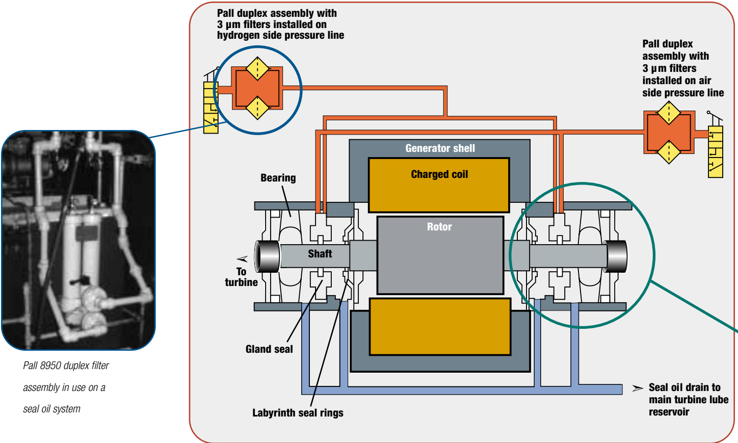
Figure 2: Diagram of a Westinghouse type seal oil system (some details have been omitted for simplification)
