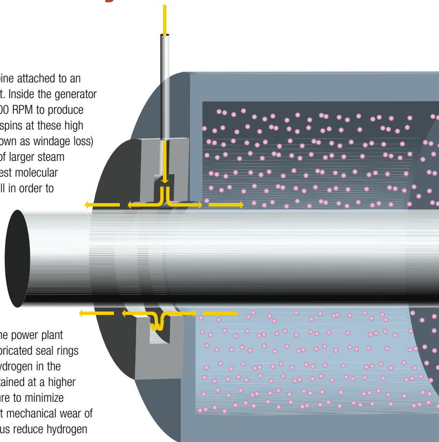
Figure 1: Oil flowing through a seal ring forms a barrier between the ring and shaft that prevents hydrogen from escaping the generator shell.
