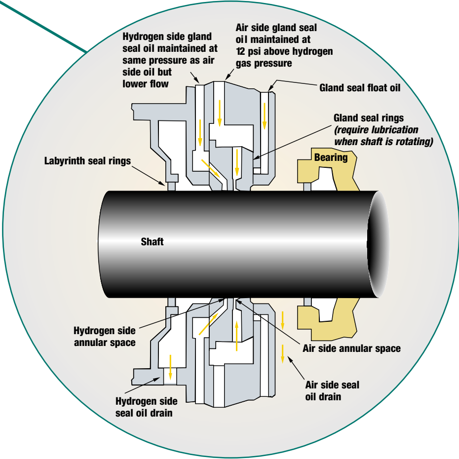
Detail of the Westinghouse type seal ring (Note separate air side and hydrogen side pressure orifices)
